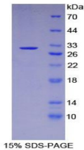
Figure. SDS-PAGE
