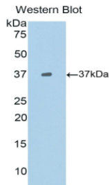
Figure. Western Blot; Sample: Recombinant BLC1, Mouse.
