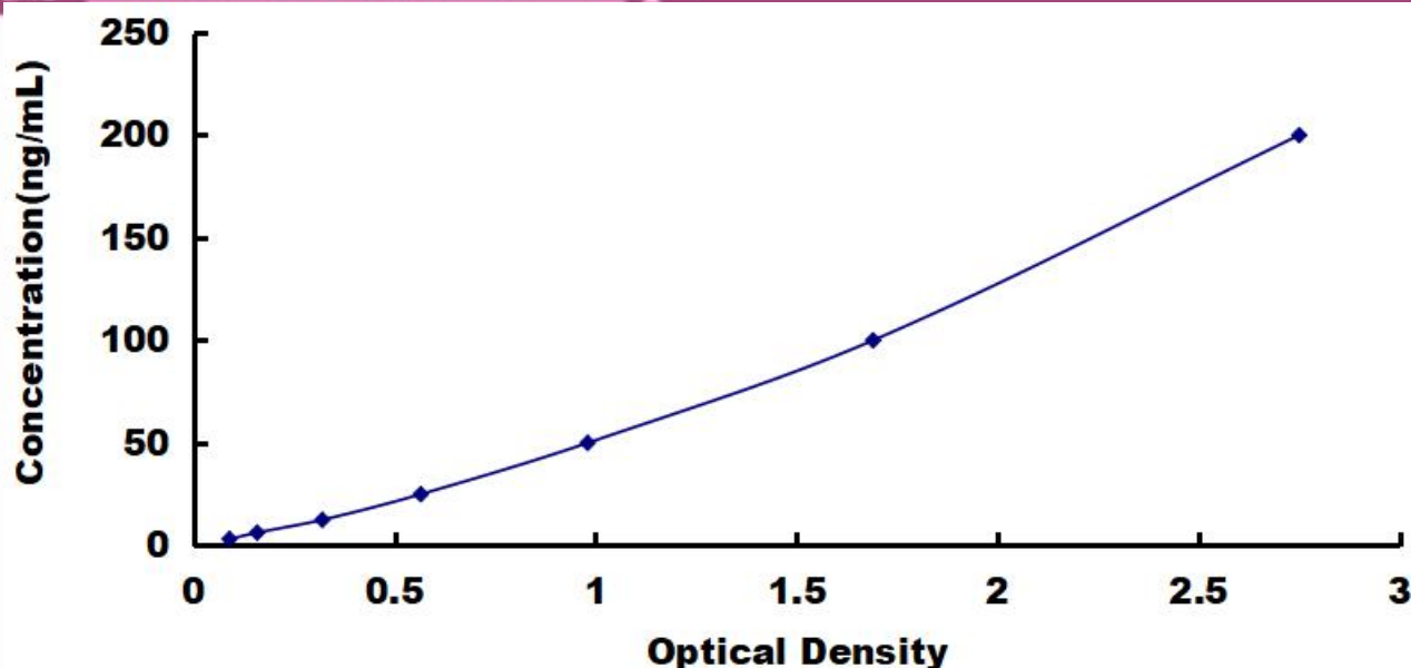
Typical Standard Curve for RBP4, Mouse ELISA.
