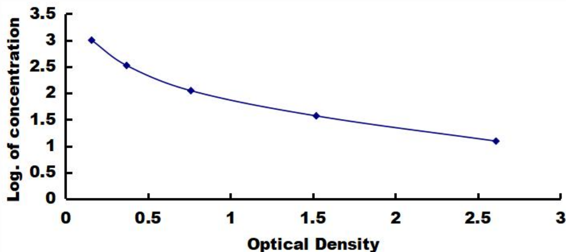
Typical Standard Curve for ACTH, Human ELISA.
