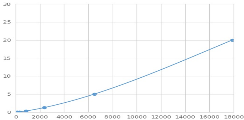
Typical Standard Curve for ZBED3 Magnetic Luminex Assay.
