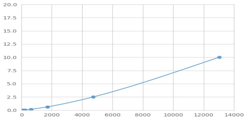
Typical Standard Curve for LYN Magnetic Luminex Assay.
