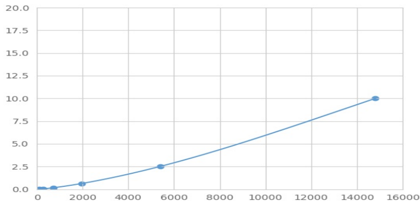
Typical Standard Curve for UGT2B7 Magnetic Luminex Assay.
