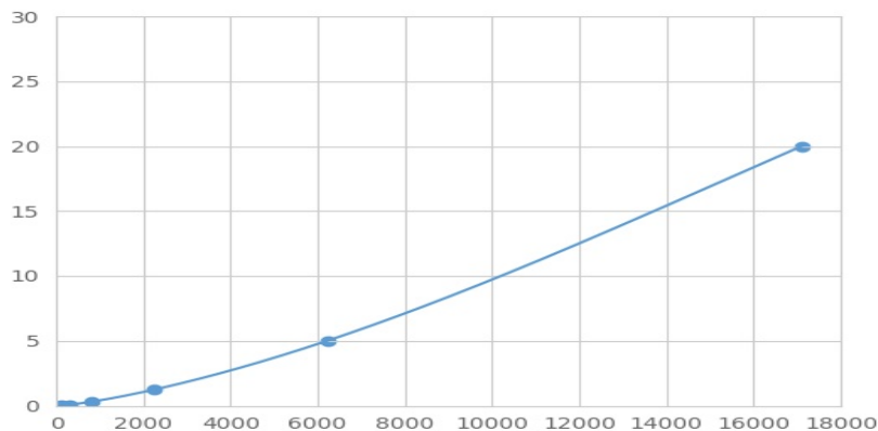
Typical Standard Curve for SOCS2 Magnetic Luminex Assay.
