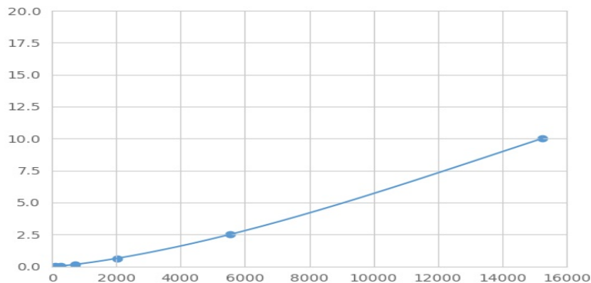
Typical Standard Curve for SLC30A4 Magnetic Luminex Assay.
