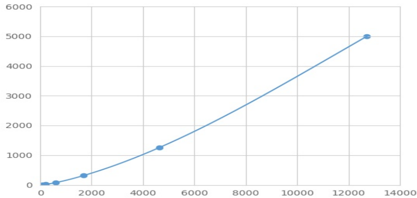
Typical Standard Curve for RGS19 Magnetic Luminex Assay.
