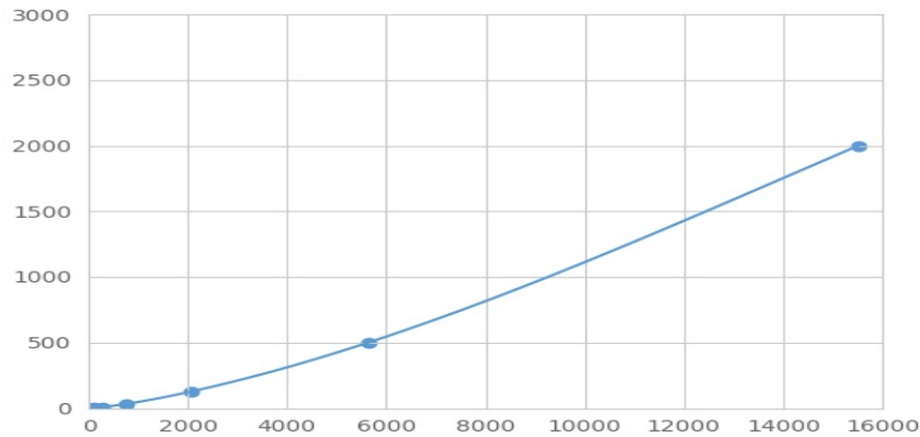
Typical Standard Curve for PPL Magnetic Luminex Assay.
