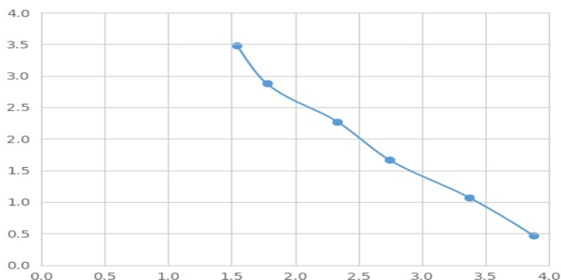
Typical Standard Curve for PTMS Magnetic Luminex Assay.
