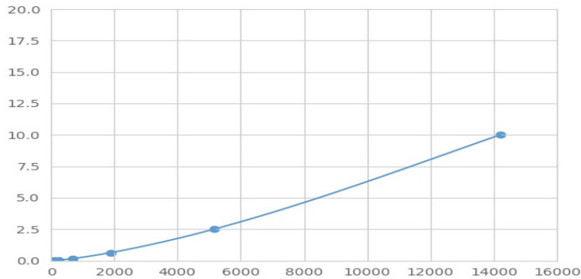
Typical Standard Curve for NANOG Magnetic Luminex Assay.
