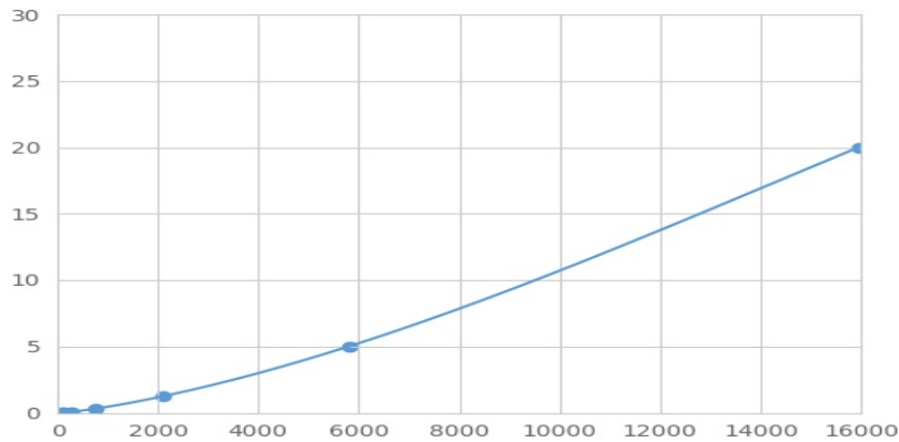
Typical Standard Curve for HSPA12B Magnetic Luminex Assay.
