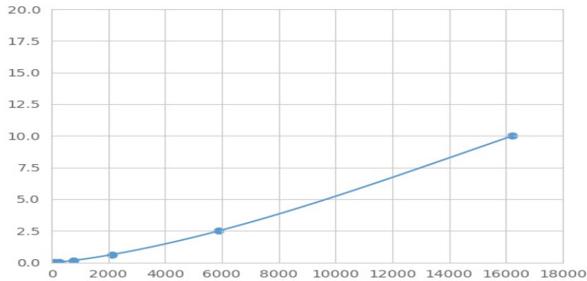
Typical Standard Curve for HAND2 Magnetic Luminex Assay.
