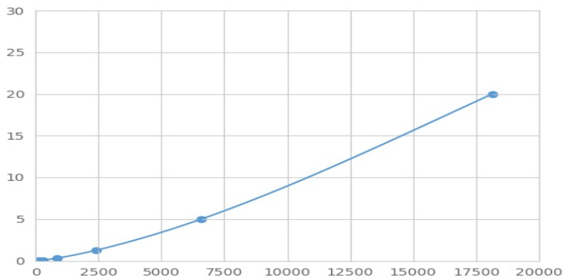
Typical Standard Curve for EAAT3 Magnetic Luminex Assay.
