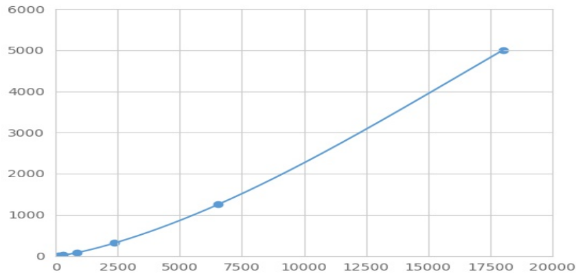
Typical Standard Curve for ENTPD3 Magnetic Luminex Assay.
