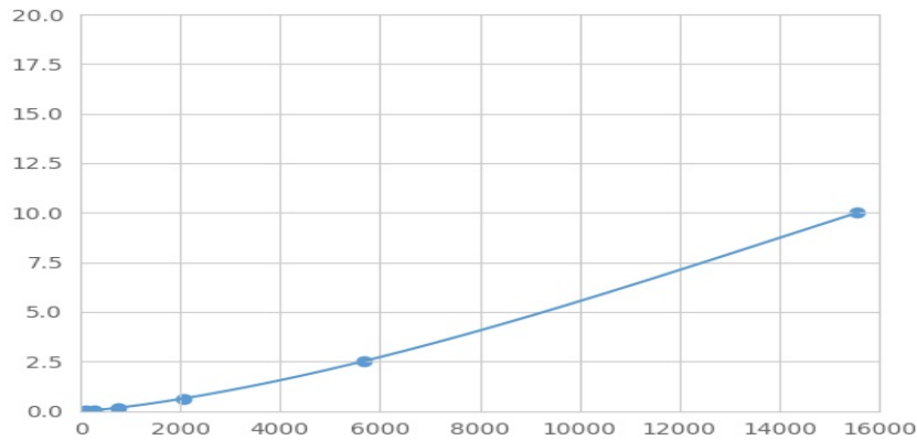
Typical Standard Curve for DAPP1 Magnetic Luminex Assay.
