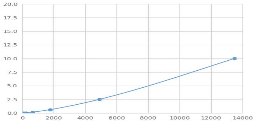
Typical Standard Curve for AHNAK Magnetic Luminex Assay.
