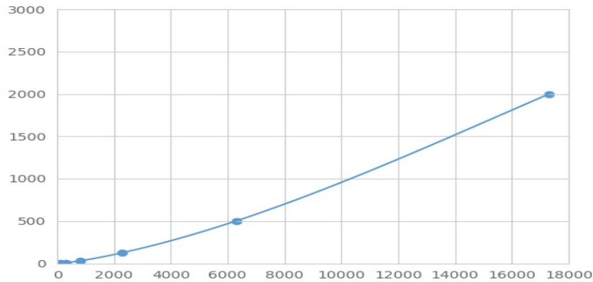
Typical Standard Curve for CDK16 Magnetic Luminex Assay.
