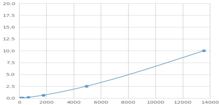
Typical Standard Curve for CTHRC1 Magnetic Luminex Assay.
