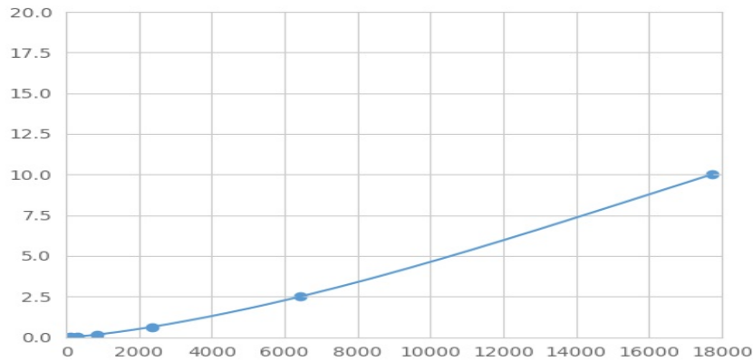
Typical Standard Curve for CLDN6 Magnetic Luminex Assay.
