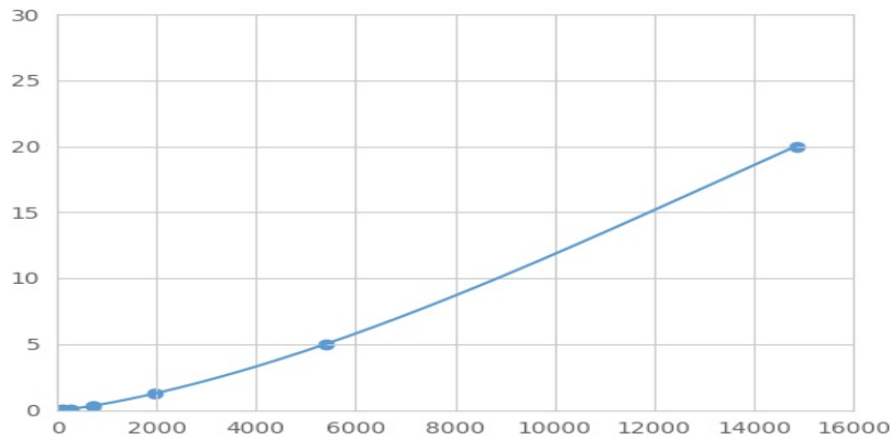
Typical Standard Curve for BIRC6 Magnetic Luminex Assay.
