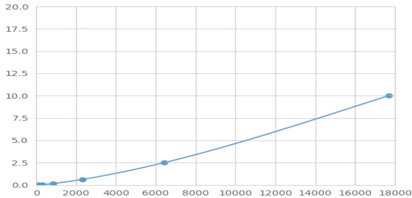
Typical Standard Curve for ADORA3 Magnetic Luminex Assay.
