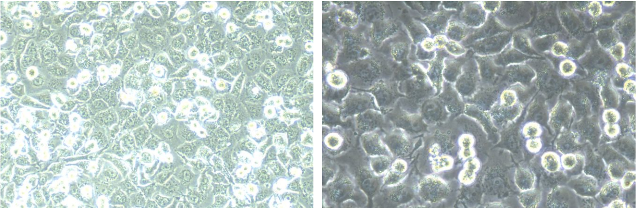
Morphology of NCI-H2030 (Optical microscope, 100x, 200x)
