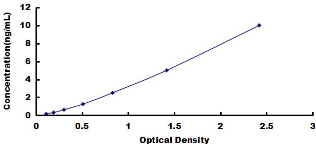
Typical Standard Curve for MAPt, Mouse ELISA.
