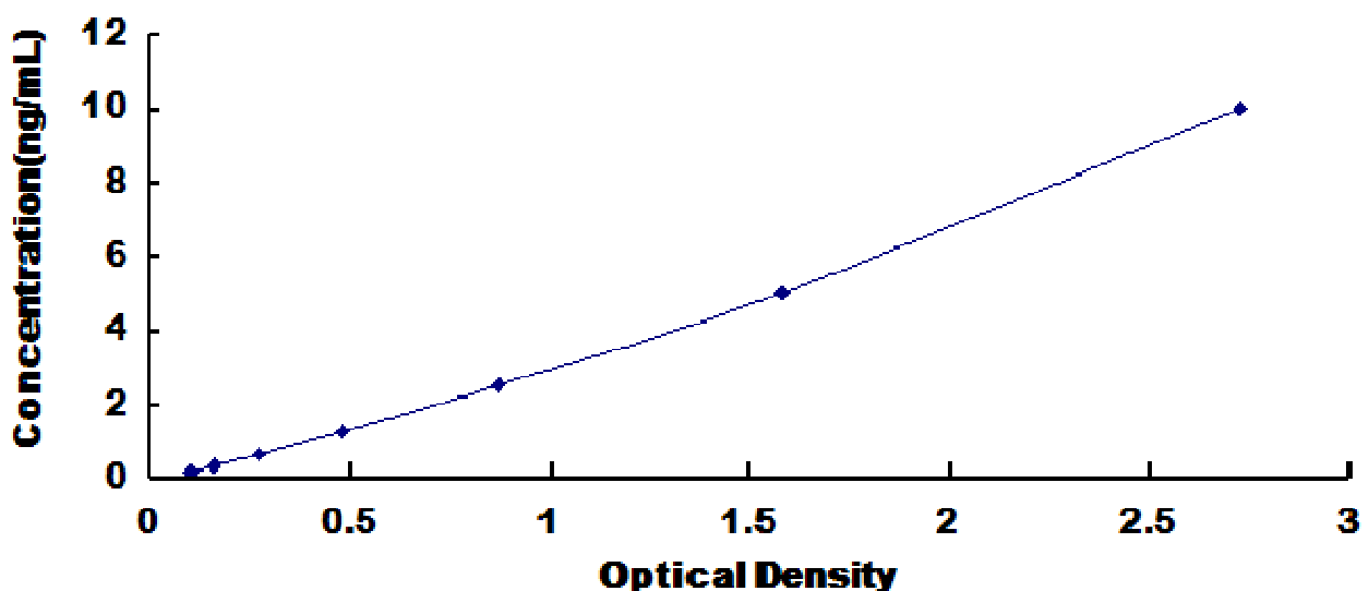
Typical Standard Curve for SLC30A4, Mouse ELISA.
