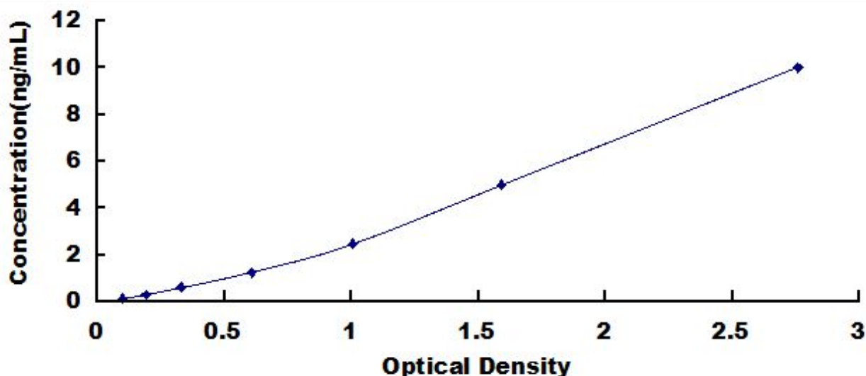
Typical Standard Curve for SPP2, Mouse ELISA.
