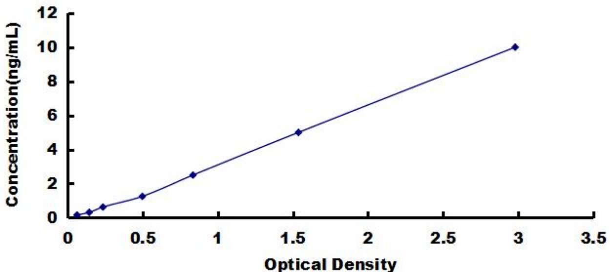
Typical Standard Curve for Podocalyxin, Mouse ELISA.
