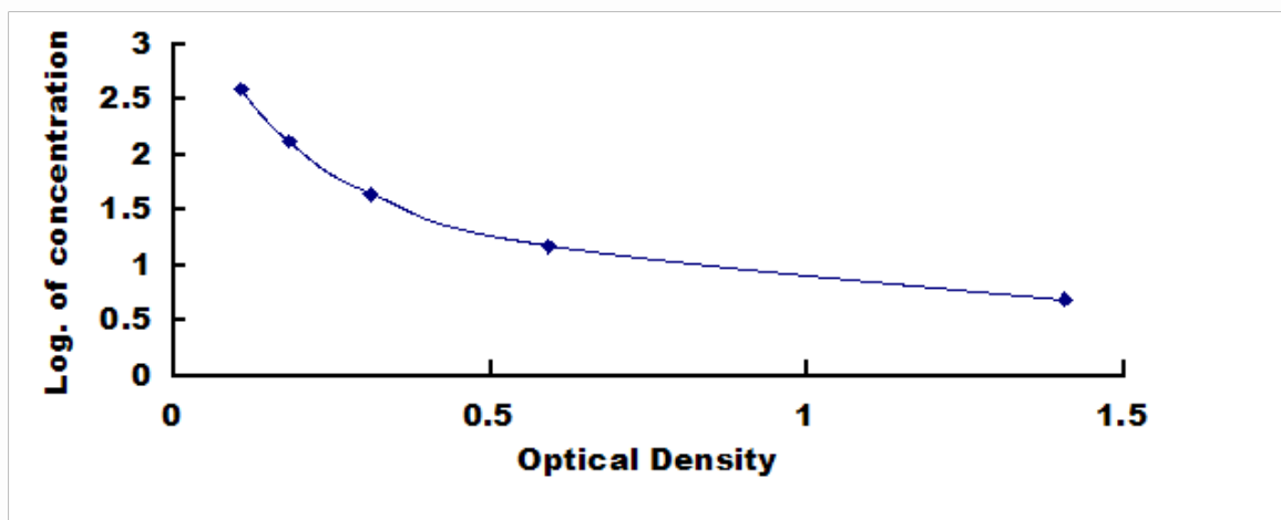
Typical Standard Curve for Pentosidine ELISA.
