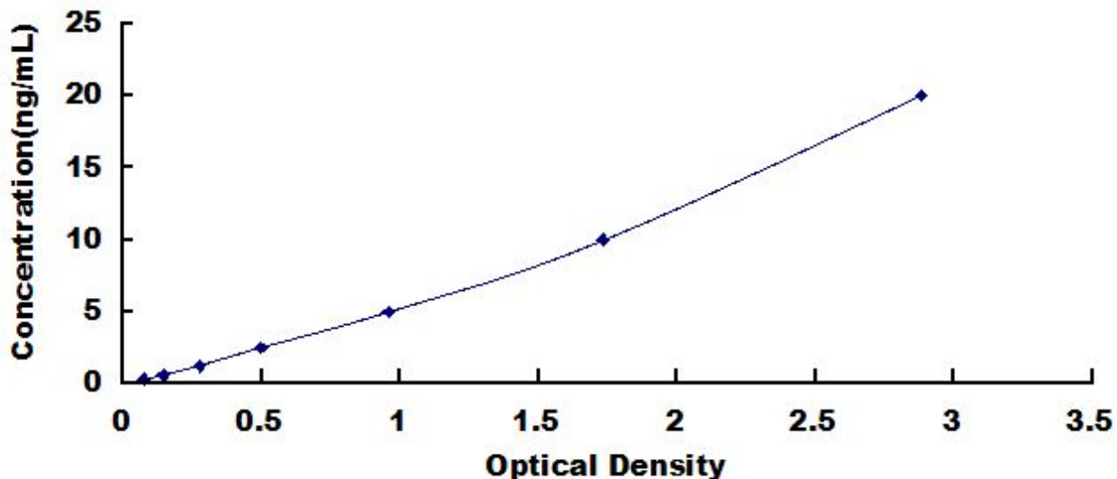
Typical Standard Curve for NPM1, Mouse ELISA.
