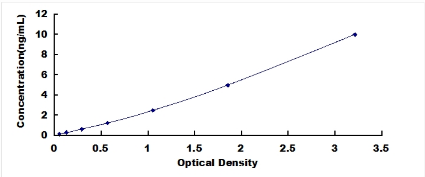
Typical Standard Curve for NEK7, Human ELISA.
