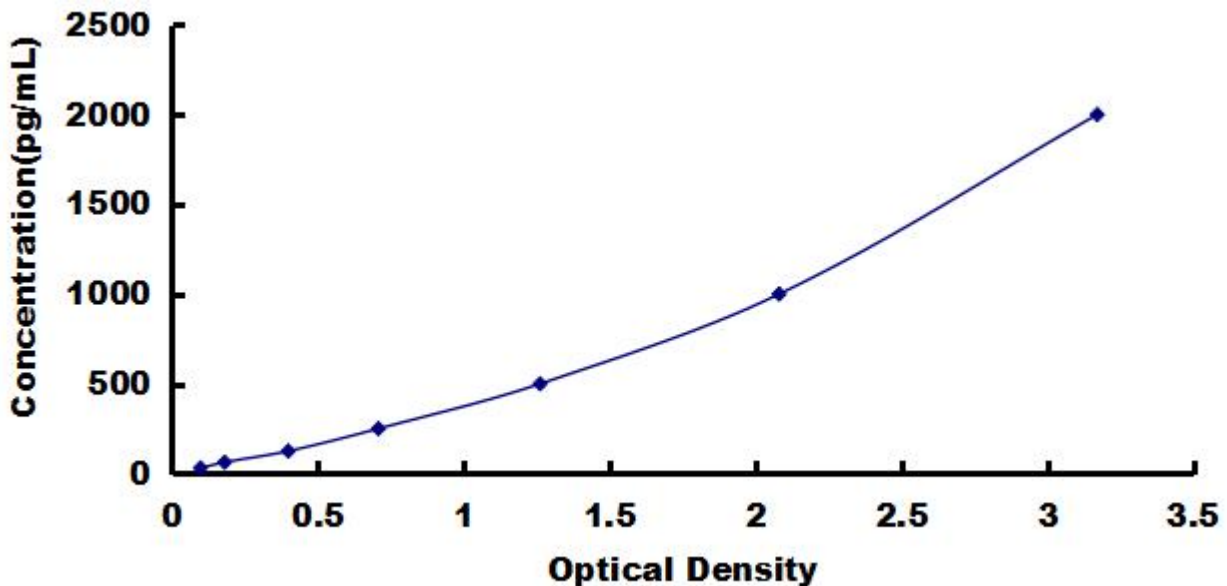
Typical Standard Curve for IL1RA, Canine ELISA.
