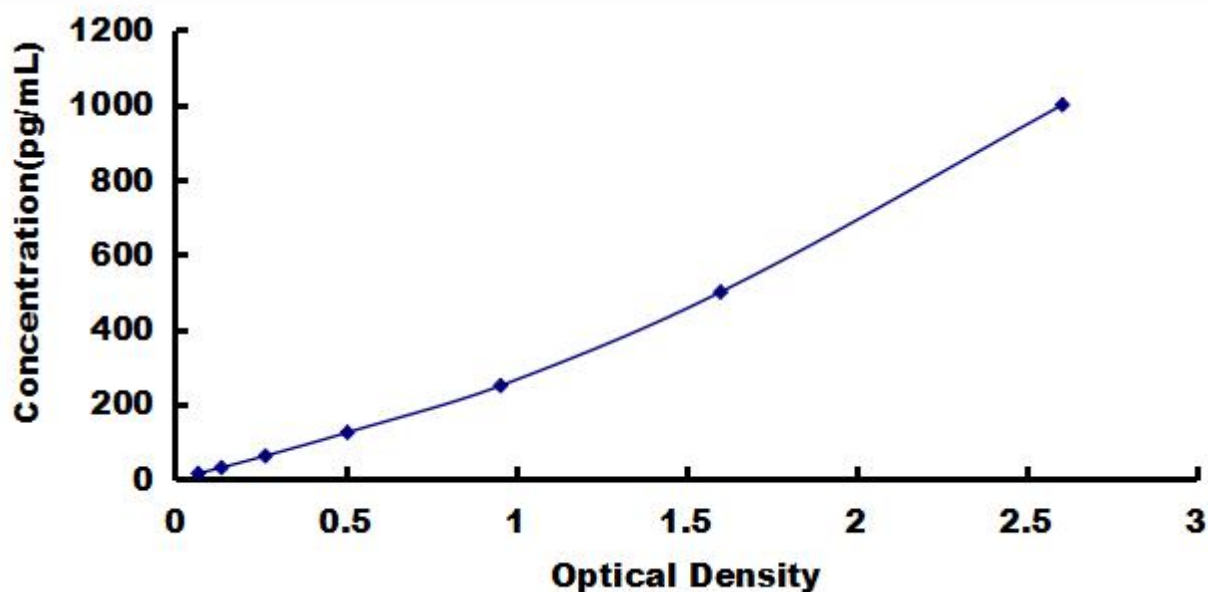
Typical Standard Curve for IL1b, Fish ELISA.
