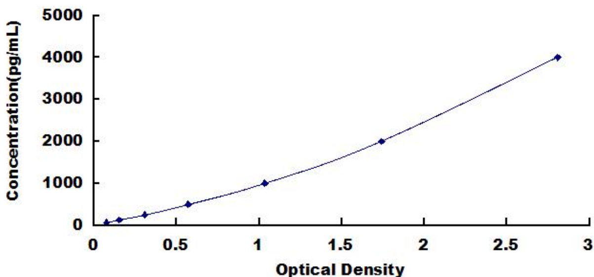
Typical Standard Curve for HMG1, Human ELISA.
