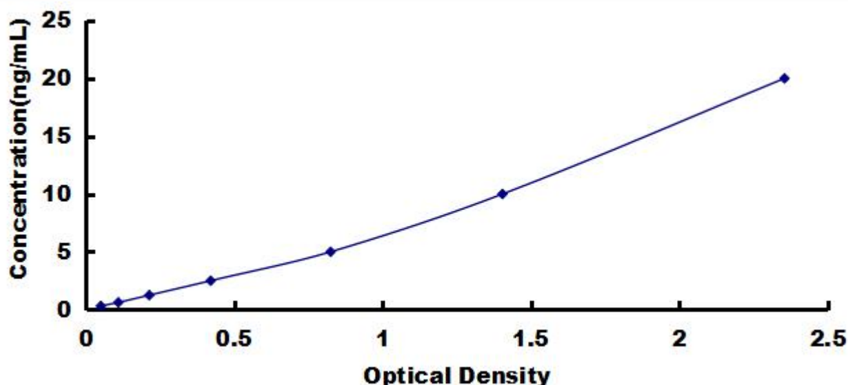
Typical Standard Curve for FBP2, Human ELISA.
