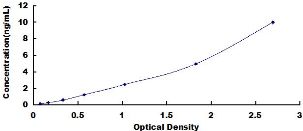
Typical Standard Curve for Ferroportin, Mouse ELISA.
