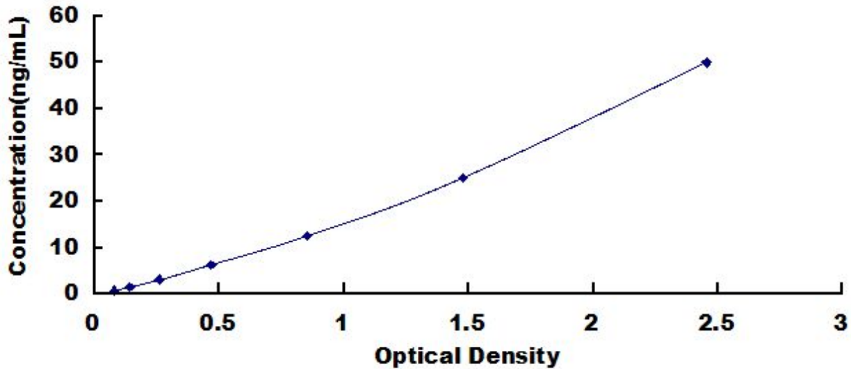
Typical Standard Curve for FABP1, Gallus ELISA.
