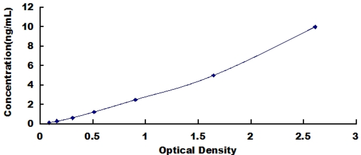
Typical Standard Curve for DOT1L, Human ELISA.
