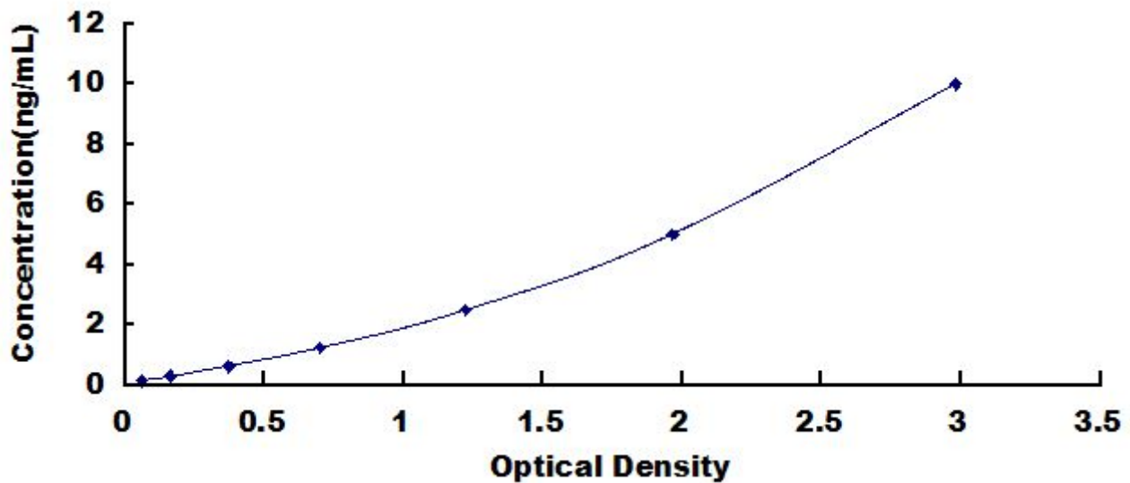
Typical Standard Curve for ConA ELISA.
