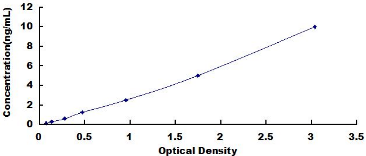
Typical Standard Curve for CTSF, Mouse ELISA.
