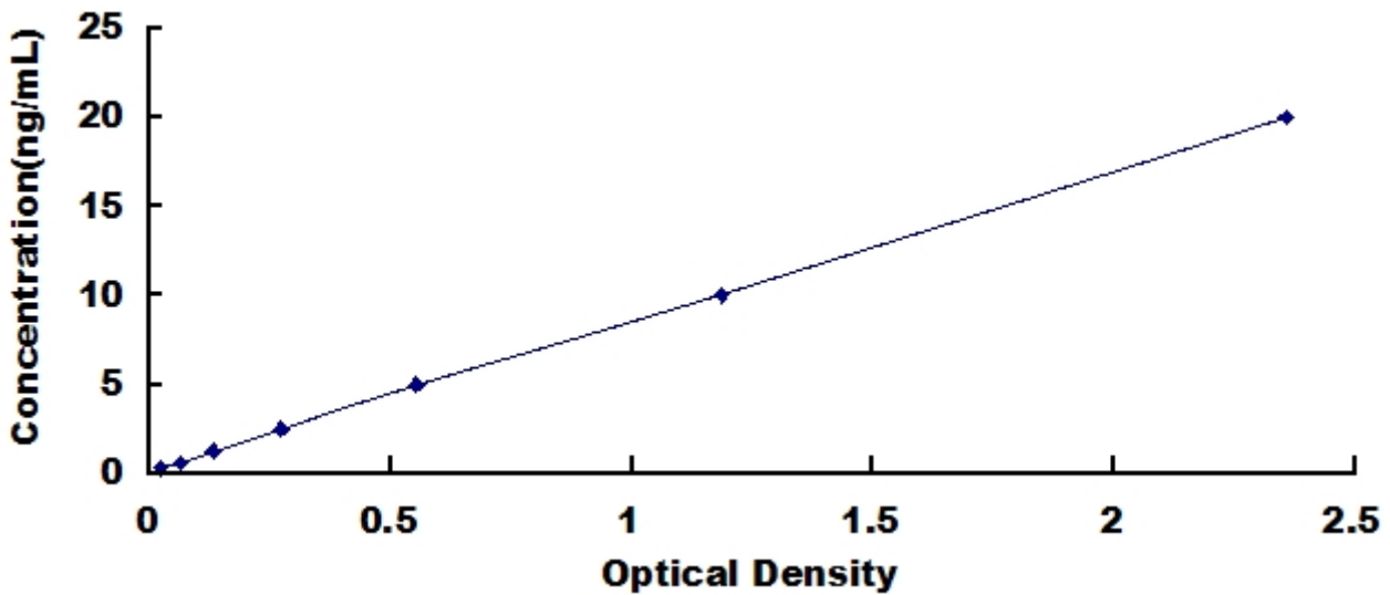
Typical Standard Curve for CLSTN3, Rat ELISA.
