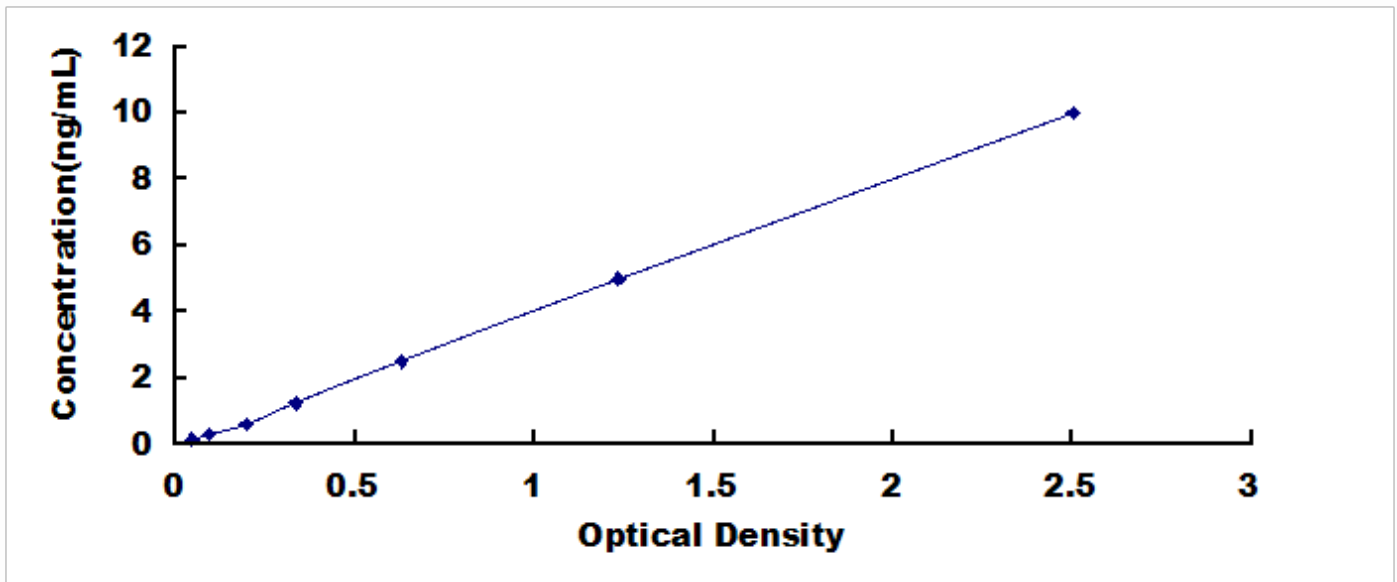
Typical Standard Curve for CAMKK2, Human ELISA.
