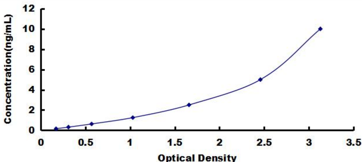
Typical Standard Curve for CLEC4D, Human ELISA.
