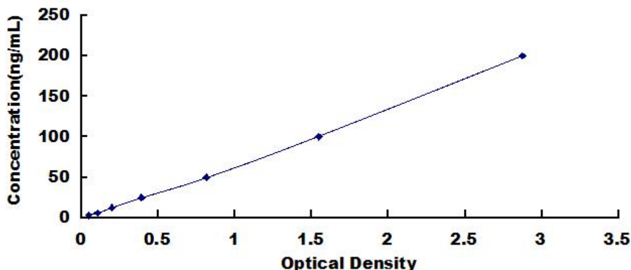
Typical Standard Curve for Anti-TG, Human ELISA.
