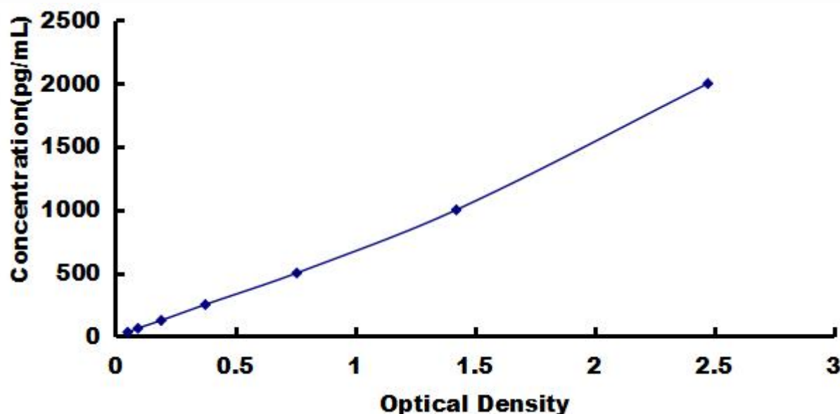
Typical Standard Curve for Anti- BRCA2, Human ELISA.
