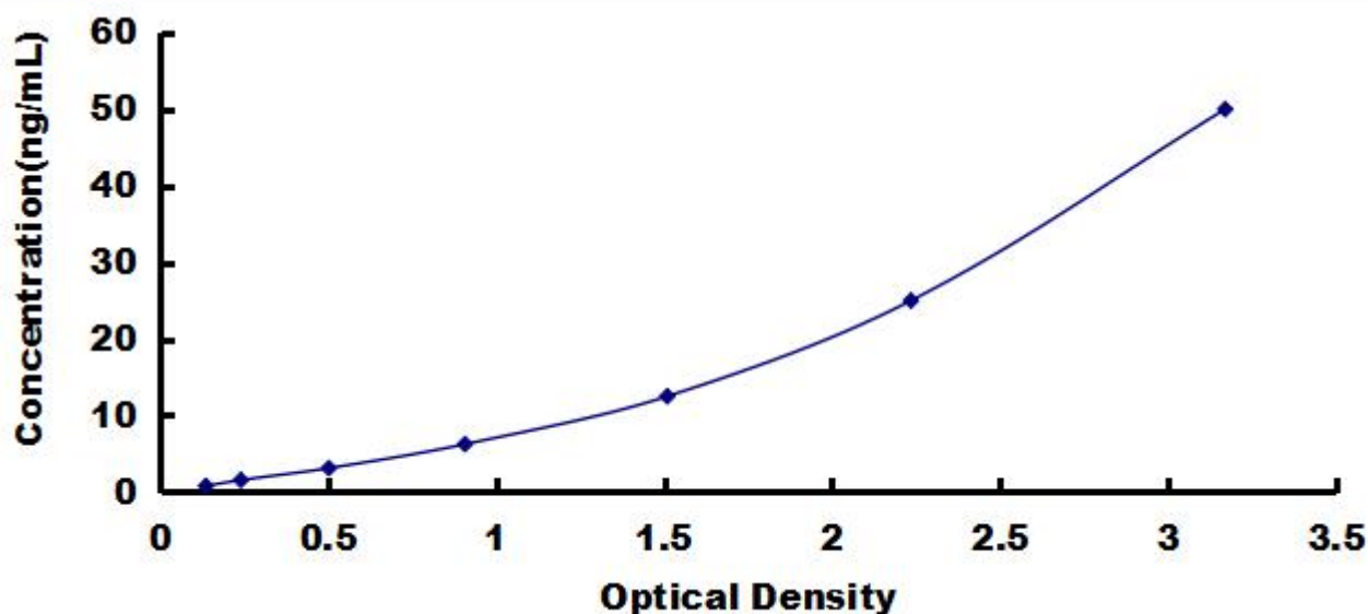
Typical Standard Curve for Adiponectin, Bovine ELISA.
