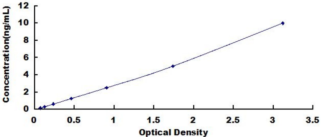
Typical Standard Curve for ADAR, Human ELISA.
