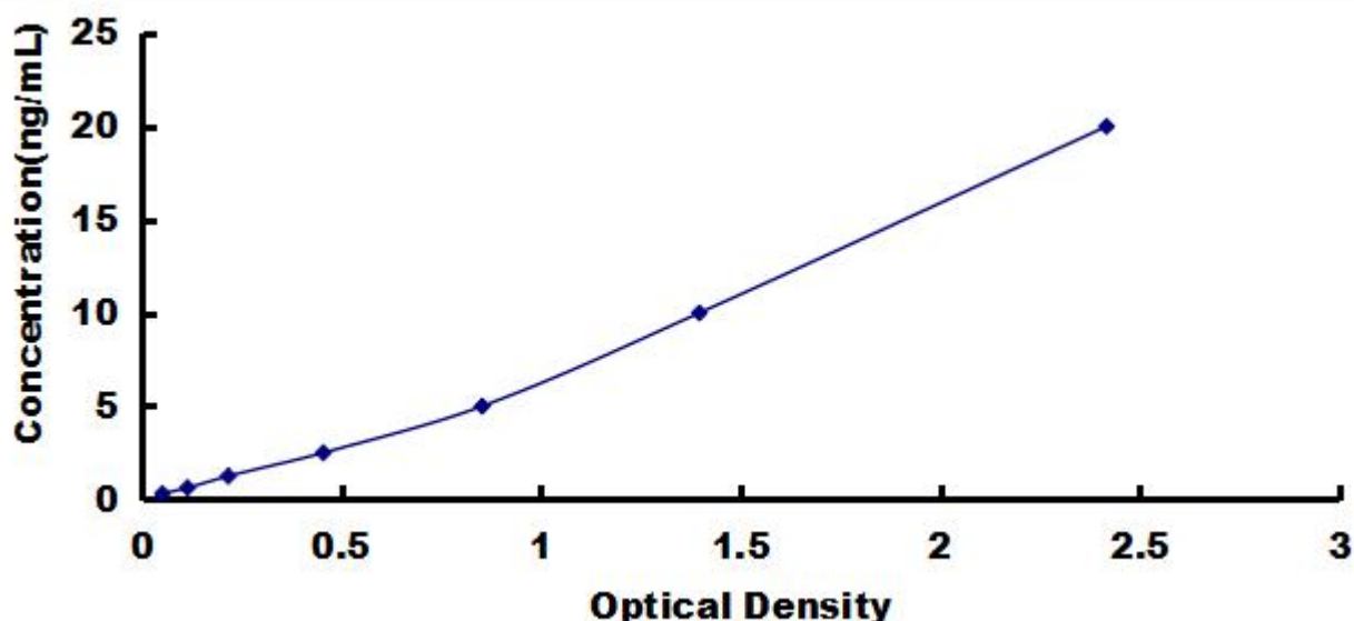
Typical Standard Curve for ADAMTS2, Human ELISA.
