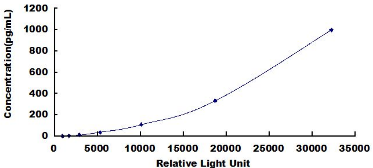
Typical Standard Curve for IL17B, Mouse CLIA.
